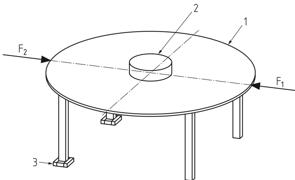
f) Cantilever table – third and fourth directions
