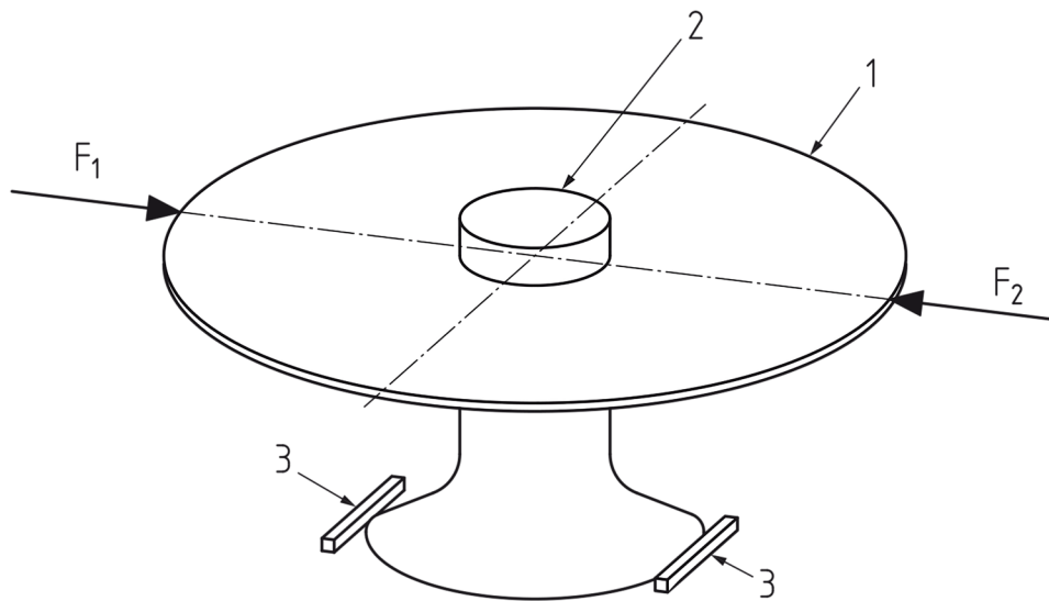
h) Oval/round table – third and fourth directions
