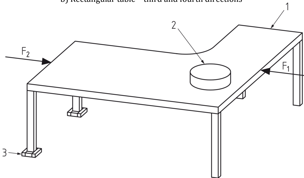
b) Rectangular table - third and fourth directions
