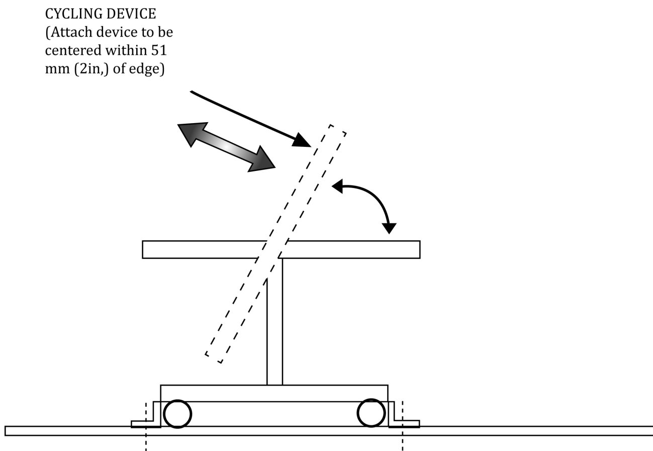
Figure 16 — Tilting Top Table - Cycle Test
