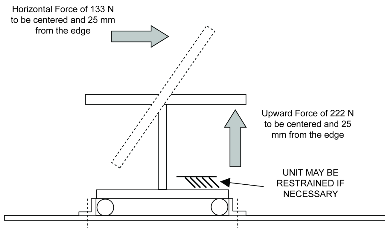
Figure 17 — Tilting Top Table - Latch Strength Test
