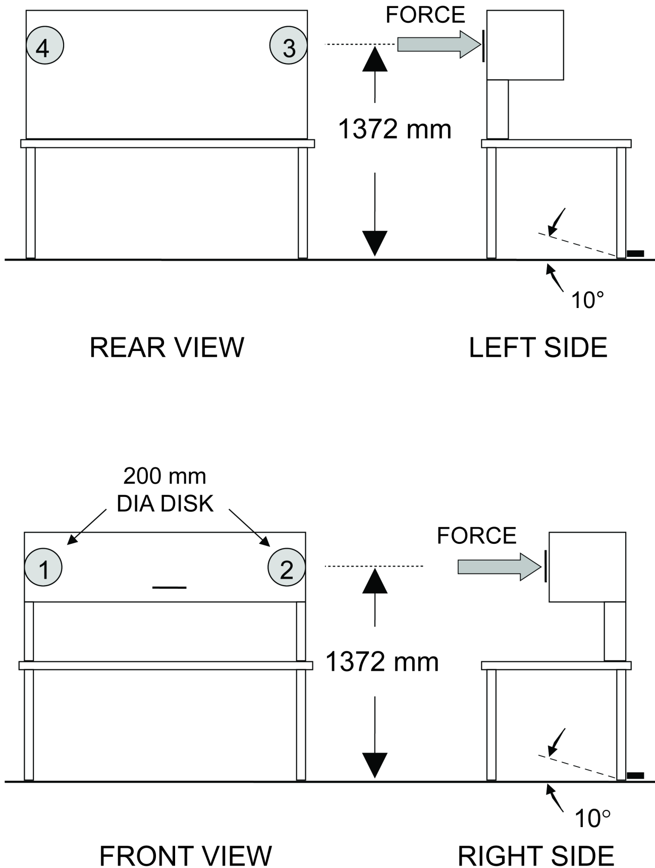
Figure 14 — Force Stability Test for Tall Products
